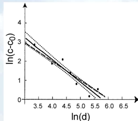
Fig. 2: The experimental (solid line) and theoretical (dashed line) dependencies of the average total number concentration (in \text{cm}^{-3} ) with deducted background ( c - c_0 ) at a distance from the middle of the road (in meters). The dotted curves give the standard errors for the experimental (solid) line of the measurements taken on 30 July 2002 – see also Table 1.
