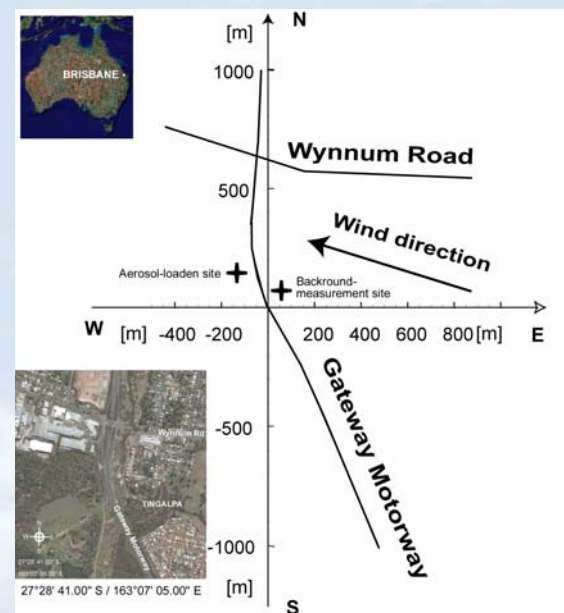
Fig. 1: The area of measurements near Gateway Motorway, Brisbane, Australia. The indicated receptor point is at the distance ~ 60 m from the curb of the road. The scale of the map and the direction to the North are as indicated (the distances on the axes are given in meters). The cross indicates the receptor point. The insert presents a section of the map with the area of measurements.
